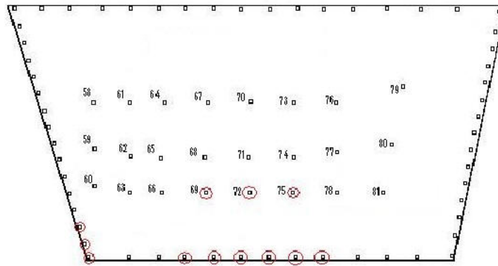
Diagram showing steel-column arrangement in WTC 7, view looking down on the roof. Circled columns were possibly damaged due to debris from WTC 1 collapse, some 350 feet away (NIST, 2005) so the damage was clearly non-symmetrical, and evidently, none of the core columns was severed by falling debris. WTC 7 was never hit by a plane.
