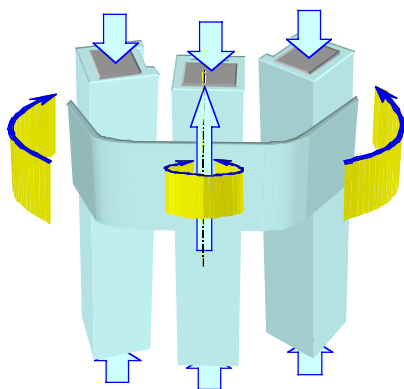
Figure 5. In a gravity collapse, the outer columns are essentially subjected to no loading in this direction.
